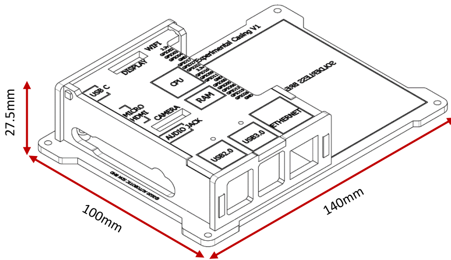
Figure 2: Overall Dimensions of Raspberry Pi 4 Acrylic Casing
